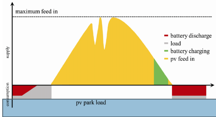
Fig. 8. Working principle of the PV and SP standby supply (nighttime) use case
