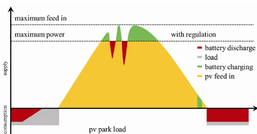
Fig. 9. Working principle of the curtailment use case
