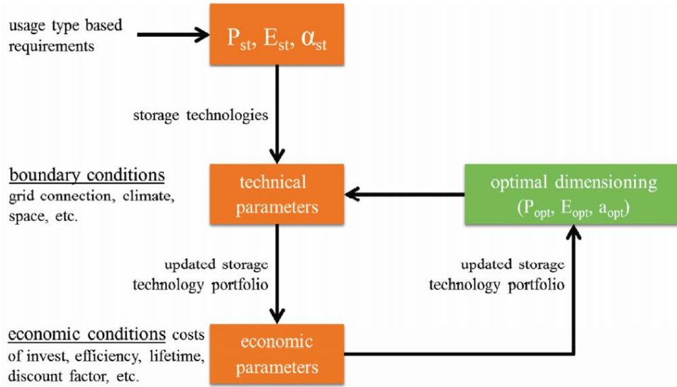
Fig. 3. Storage system sizing procedure
