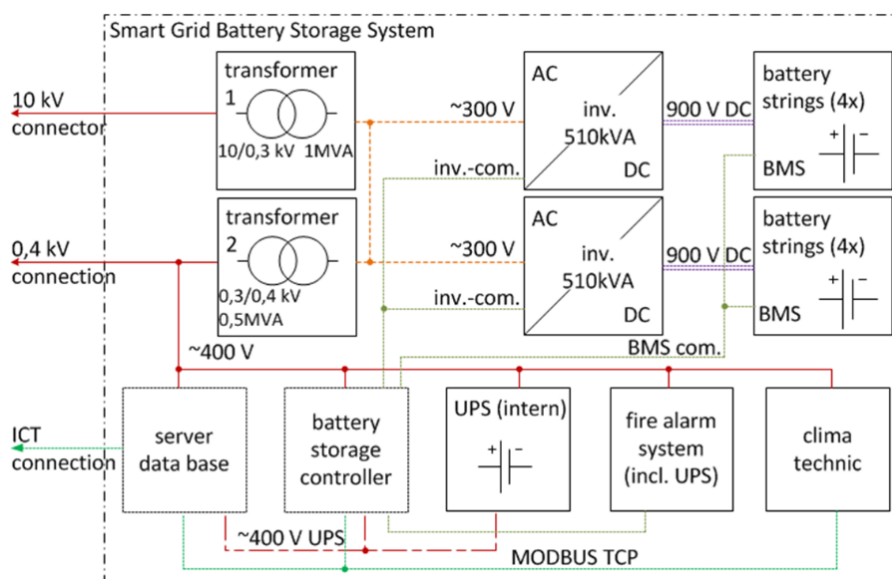
Fig. 7. SGEES circuit diagram
